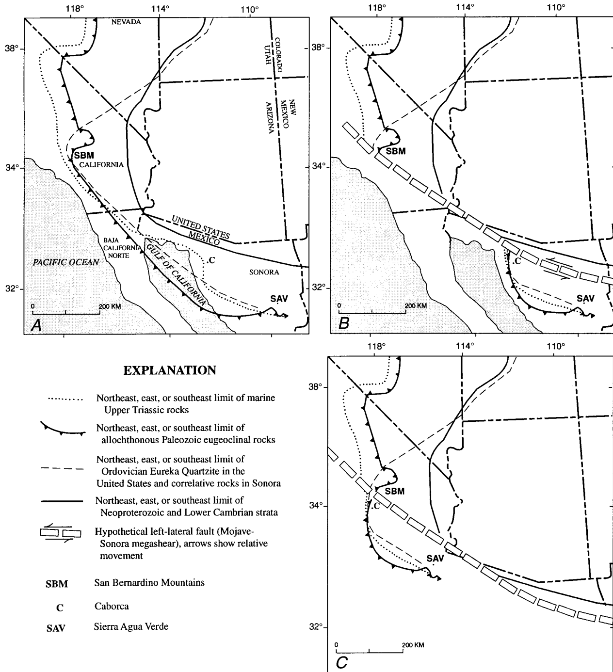
Figure 11. Tectonic and paleogeographic models of Paleozoic rocks in the western United States and northern Mexico. A, model in which the Mojave-Sonora megashear does not exist; B, model in which Paleozoic and Triassic rocks have been offset 600 km left laterally from an original position near the San Bernardino Mountains; C, palinspastic reconstruction on faults or structures other than Mojave-Sonora megashear not shown.
