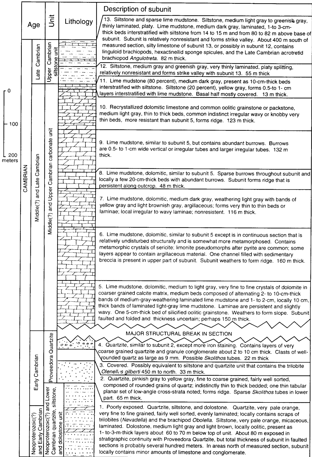
Figure 5. Lithologic column and description of Neoproterozoic (?) and Cambrian quartzite, siltstone, and dolostone unit; Lower Cambrian Proveedora Quartzite; Middle (?) and Upper Cambrian carbonate unit; and Upper Cambrian siltstone unit in Sierra Agua Verde.
