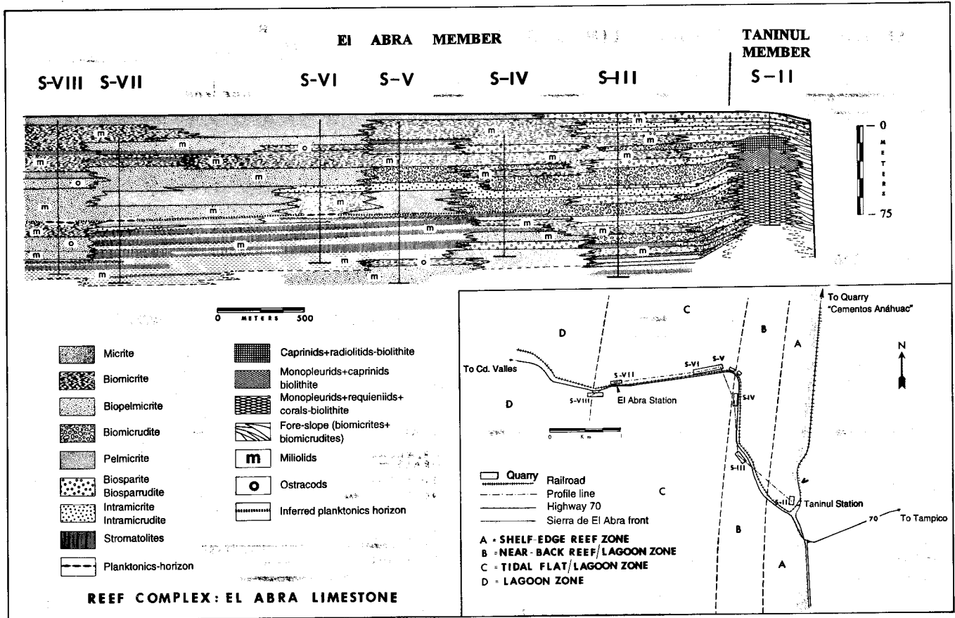
Figure 4. Stratigraphic cross-section of the reef complex El Abra Limestone in quarry exposures at its type locality.
