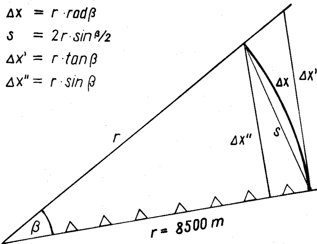
Figure 6.- Modeling of the gradual shortening increase of the Xilitla Thrust between the Tancuilín River and the Arroyo Seco section (distance r ) as a rigid-body rotation (with the angle \beta ) around the southern tip of the thrust. \Delta x = displacement-path curve for point A. Note that measuring the shortening normal to the structural trend, either too great ( \Delta x' ) or too small ( \Delta x'' ) values are obtained.
