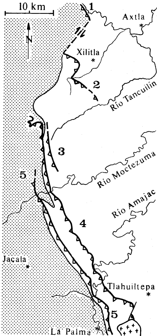
Figure 8.- Hidalgo deformations at the eastern edge of the Valles-San Luis Potosí carbonate platform. Imbricate thrust sheets (shortening 3-5 km each) formed where the bank edge was approximately normal to the early Tertiary trajectories of the maximum principal stress (as deduced from fold axes), whereas a transcurrent fault developed, where the bank edge formed an acute angle with the same stress trajectories. Dotted: Valles-San Luis Potosí Platform.
