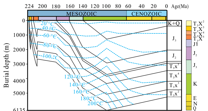
Figure 11. Burial history for well Chuanxiao565 of the WDSC.
