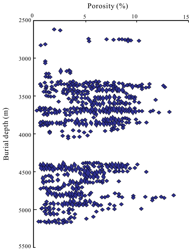
Figure 14. Porosity versus burial depth of the Xu2 sandstones, showing decreasing porosity with the increase of burial depth.
