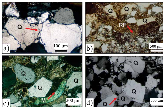
Figure 4. Photomicrographs of mechanical and chemical compaction with arrows showing the features. (a) Fracturing of brittle grains in the sandstone of well Xin853 at 3408.48 m. (b) Rock fragments and micas bent around resistant detrital grains in the sandstone of well Chuanya92 at 2796.5 m and (c) in the sandstone of well Xin853 at 3397.25 m. (d) Concave-convex grain contacts and fractures in the sandstone of well Chuanmian93 at 4056.0m. Q=quartz, RF=rock fragments, M=mica.
