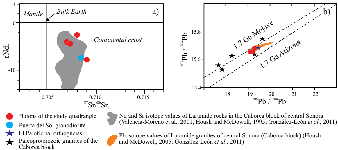
Figure 6. a) Plot of initial \epsilon Nd_i versus ^{87}Sr/^{86}Sr_i values for the El Gato, El Oquimonis, Las Mayitas and El Garambullo plutons of the Puerta del Sol area. Values plot close to the Laramide granites of the Caborca block in central Sonora (gray field) reported by other authors and summarized in González-León et al. (2011). Sr and Nd values of the Puerta del Sol granodiorite (blue dot) are from González-León et al. (2011) b) Uranogenic diagram (Wooden et al. , 1988; Wooden and DeWitt, 1991) showing plots of the El Palofierral orthogneiss and the Laramide and syn-extensional plutons of the study area. Black stars are Pb isotope values reported from Paleoproterozoic granites of the Caborca terrane by Farmer et al. (2005) and González-León et al. (2011).
