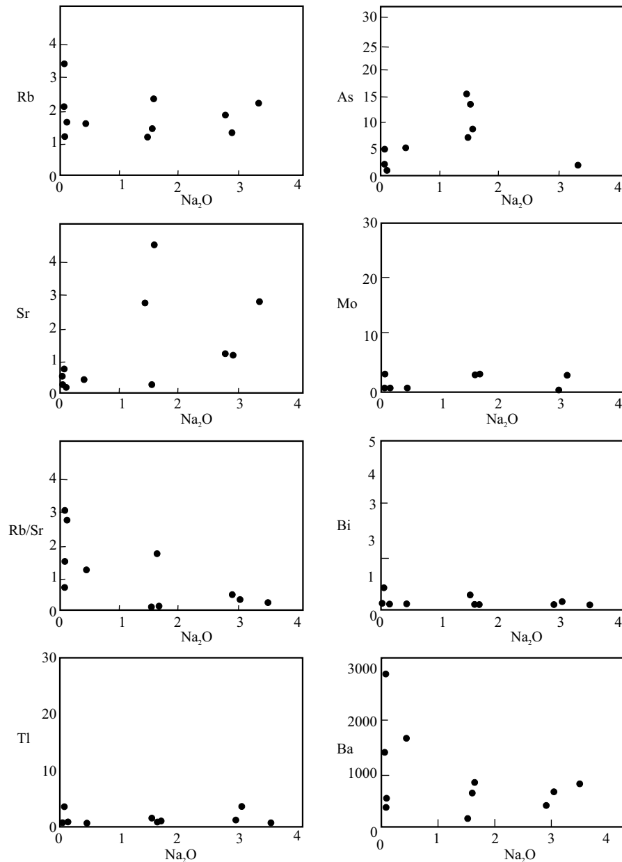
Figure 13. Variation diagrams for SAL-25 DDH showing the variability of trace element concentrations in hanging-wall rhyolite and quartz-eye porphyry (Rb, Sr, Rb/Sr, Tl, As, Mo, Bi and Ba ppm vs. Na 2 O %).
