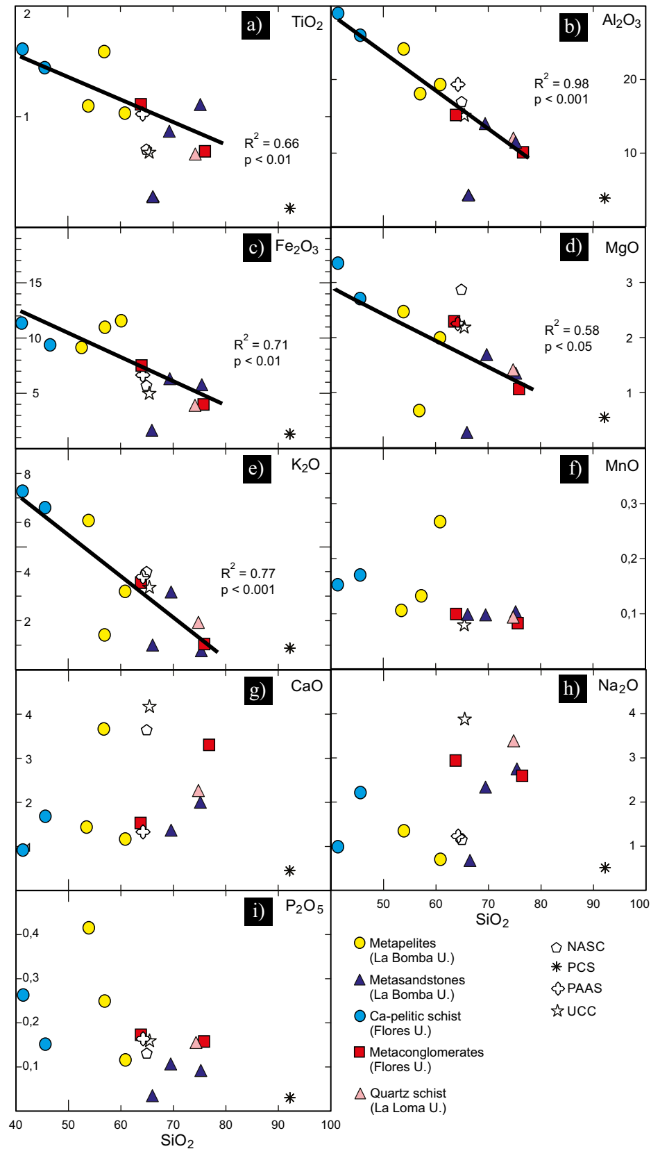
Figure 12. Chemical variation plots of metasedimentary rocks from the Difunta Correa metasedimentary sequence. Samples SPP-22013 and SPP-424 are not shown in the CaO and Na 2 O plots (respectively) because contents of these components are off-scale. Values in weight percent. Sample SPP-22013 was not considered in correlation coefficients due to their carbonaceous cement.
