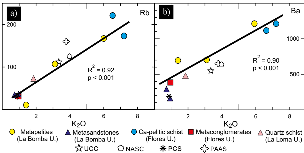
Figure 14. Variation plots of Rb and Ba of metasedimentary rocks from the Difunta Correa metasedimentary sequence. Values in weight percent for major elements and ppm for trace elements. Sample SPP-22013 was not considered in correlation coefficients due to their carbonaceous cement.
