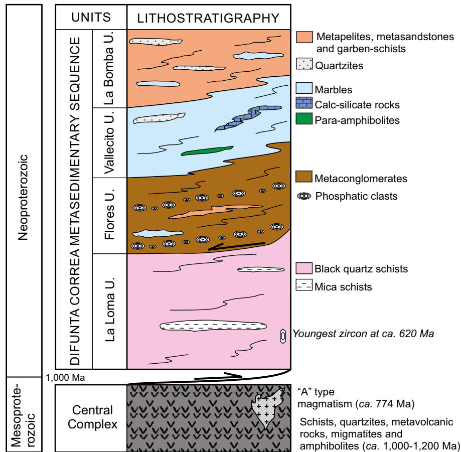
Figure 4. Schematic lithostratigraphic column of the Difunta Correa metasedimentary sequence. The youngest zircon age is from Rapela et al. (2005, 2015).
