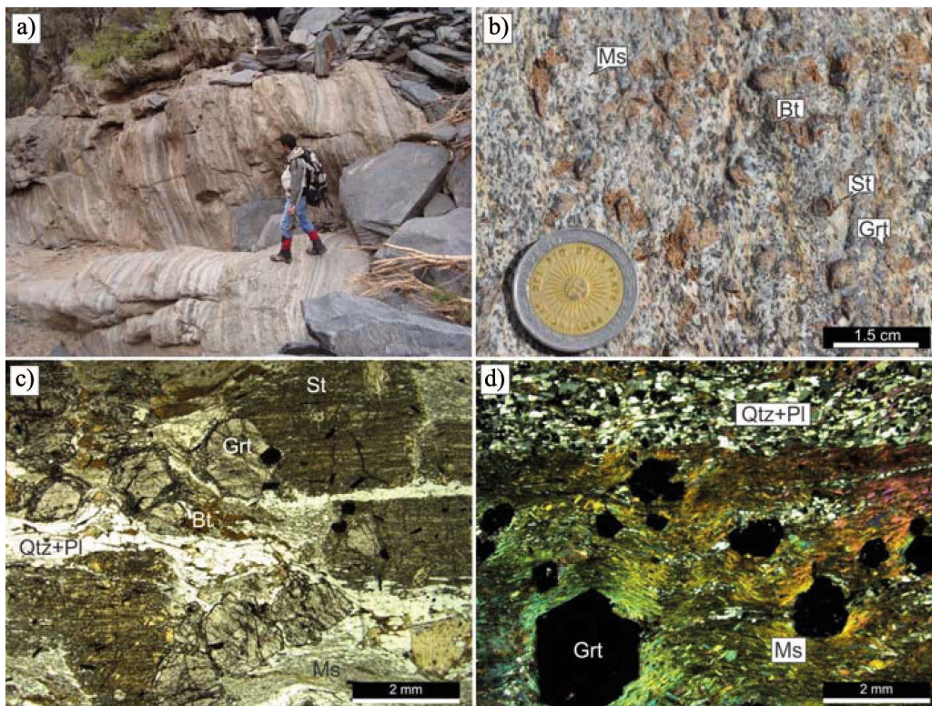
Figure 9. La Bomba unit. a) Succession of metapelites and metasediments; b) Staurolite-garnet schist; c) PPL photomicrograph of a staurolite-garnet schist; d) Crossed polars photomicrograph of a garnet schist.
