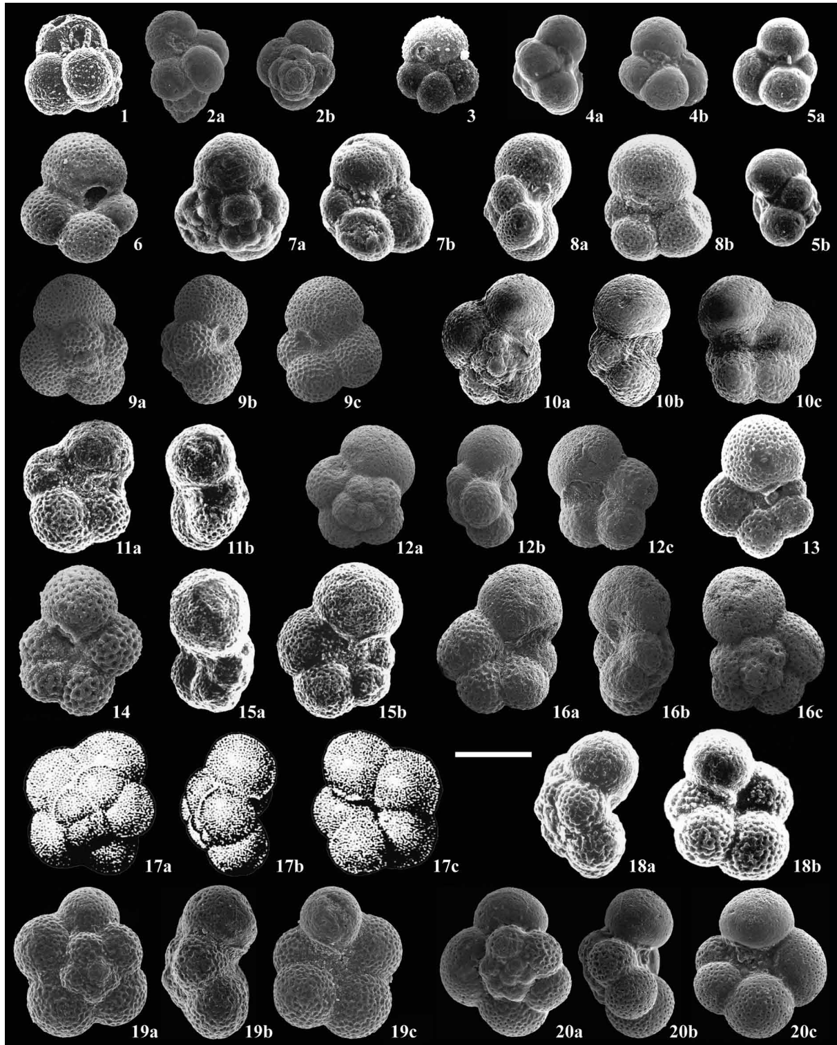
Figure 2. SEM images of Palaeoglobigerina Arenillas, Arz and Nález (2007), and Eoglobigerina Morozova (1959) species (scale bar = 100 \mu m). 1-2. Palaeoglobigerina alticonusa (Li, McGowran and Boersma, 1995): 1, holotype from Zone P \alpha , DSDP Site 152, Caribbean Pacific (from Li et al. , 1995, pl. 2, fig. 9); 2, specimen from the E. simplicissima Subzone, El Kef, Tunisia. 3-5. Palaeoglobigerina fodina (Blow, 1979): 3, holotype from Zone P \alpha , DSDP Leg 6, South Pacific (from Blow, 1979, pl. 57, figs. 5-6); 4, specimen from the Pv. longiapertura Subzone, Ain Settara, Tunisia; 5, specimen from the Pv. longiapertura Subzone, El Kef, Tunisia. 6-9. Eoglobigerina simplicissima Blow (1979): 6, holotype from Zone P \alpha , lowermost Danian, from DSDP Leg 6, South Pacific (from Blow, 1979, pl. 55, fig. 1); 7, specimen from the S. triloculinoides Subzone, Agost, Spain; 8, specimen from the E. trivialis Subzone, Ain Settara, Tunisia; 9, specimen from the E. simplicissima Subzone, Ain Settara, Tunisia. 10-13. Eoglobigerina eobulloides Morozova (1959): 10, holotype from lower Danian sediments, Tarkhankhut Peninsula, Crimea, Ukraine (from Olsson et al. , 1999, pl. 8, figs. 10-12); 11, specimen from the G. compressa Zone, Caravaca, Spain; 12, specimen from the E. simplicissima Subzone, Ain Settara, Tunisia; continues
