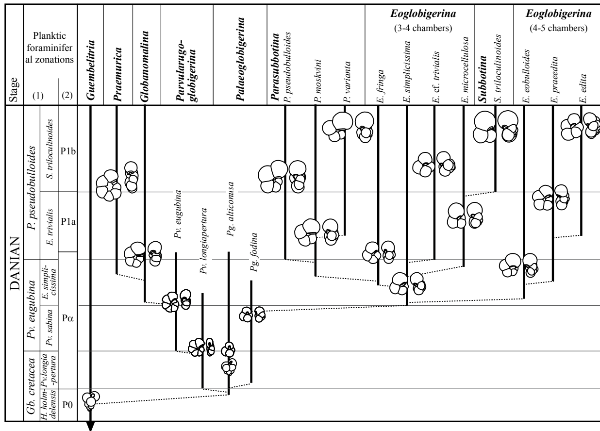
Figure 11. Proposed phylogenetic relationship of the lineage Guembeltria Cushman (1933) - Palaeoglobigerina Arenillas, Arz and Nández (2007) - Parvularugoglobigerina Hofker (1978) - Globanomalina Haque (1956) - Praemurica Olsson, Hemleben, Berggren and Liu (1992) are based on Arenillas et al. (2007, 2010).
