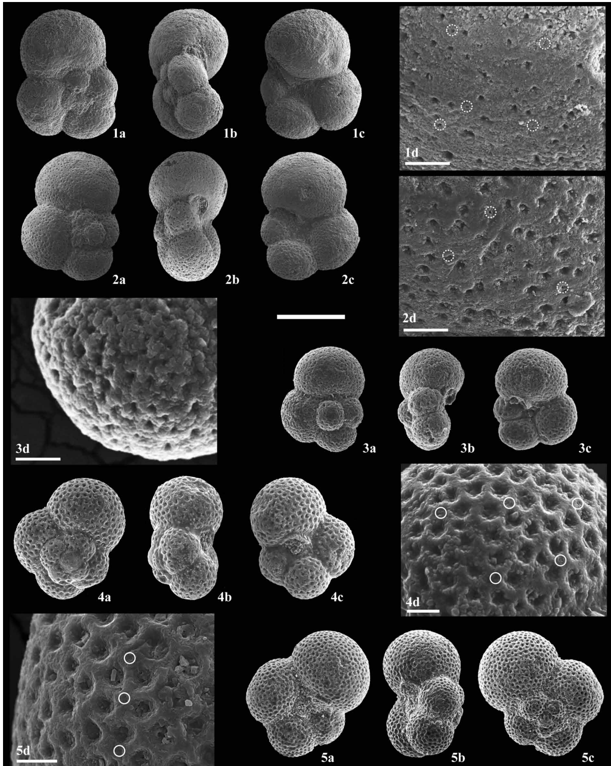
Figure 6. SEM images of Eoglobigerina simplicissima and Eoglobigerina fringa specimens and details of their smooth wall texture (scale bar = 100 \mu\text{m} ; scale bar of wall details = 10 \mu\text{m} ). 1-3. Eoglobigerina simplicissima Blow (1979): 1, specimen intermediate to Pg. fodina , from the E. simplicissima Subzone, El Kef, Tunisia; 2, specimen intermediate to Pg. fodina , from the E. simplicissima Subzone, El Kef, Tunisia; 3, juvenil specimen from the E. simplicissima Subzone, El Kef, Tunisia. 4-5. Eoglobigerina fringa (Subbotina, 1950): 4, specimen intermediate to E. simplicissima , from the E. simplicissima Subzone, El Kef, Tunisia; 5, specimen from the S. triloculinooides Subzone, Ben Gurion, Israel. Dashed circles mark possible spine holes and solid circles probable or certain spine holes.
