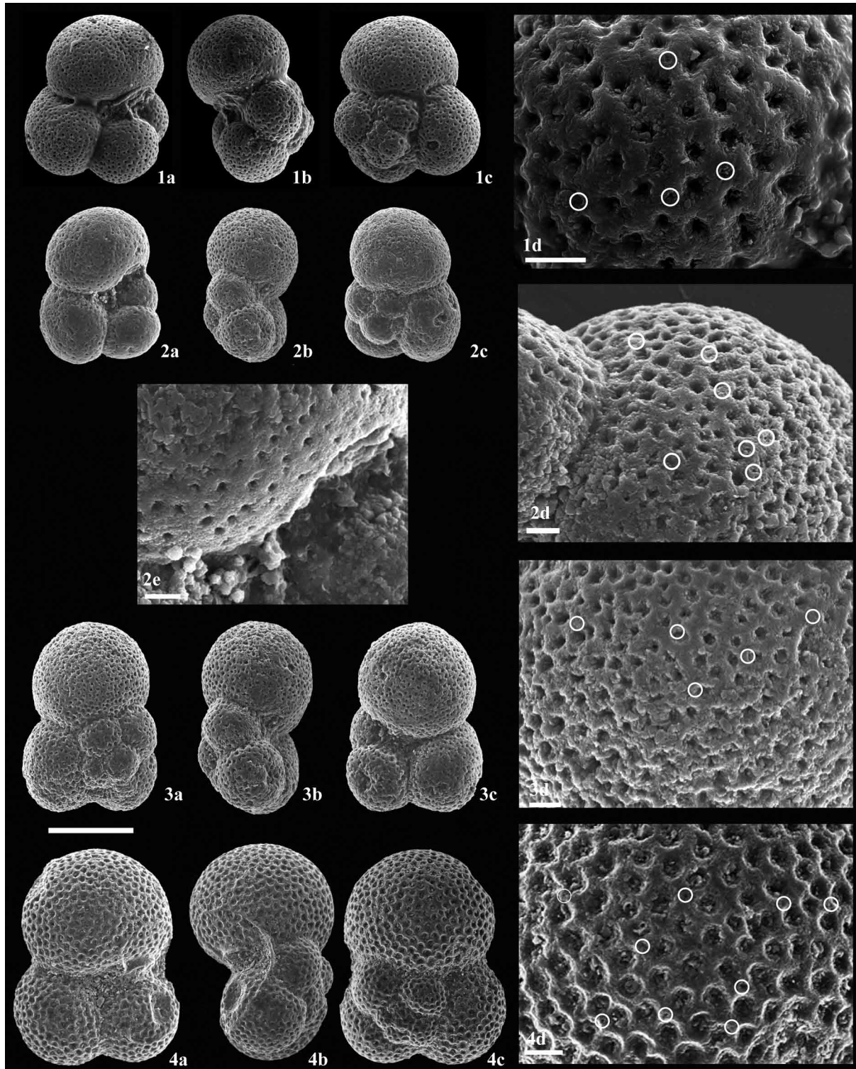
Figure 9. SEM images of Eoglobigerina simplicissima , Eoglobigerina microcellulosa and Subbotina triloculinoidea specimens and details of their smooth wall texture; possible spine holes surrounded with white circles (scale bar = 100 \mu m; scale bar of wall details = 10 \mu m). 1. Eoglobigerina simplicissima Blow (1979): specimen from the E. simplicissima Subzone, El Kef, Tunisia. 2-3. Eoglobigerina microcellulosa (Morozova, 1961): 2, specimen from the E. simplicissima Subzone, El Kef, Tunisia; 3, specimen from the E. simplicissima Subzone, El Kef, Tunisia. 4. Subbotina triloculinoidea (Plummer, 1927): specimen from the S. triloculinoidea Subzone, Ben Gurion, Israel. Solid circles mark probable or certain spine holes.
