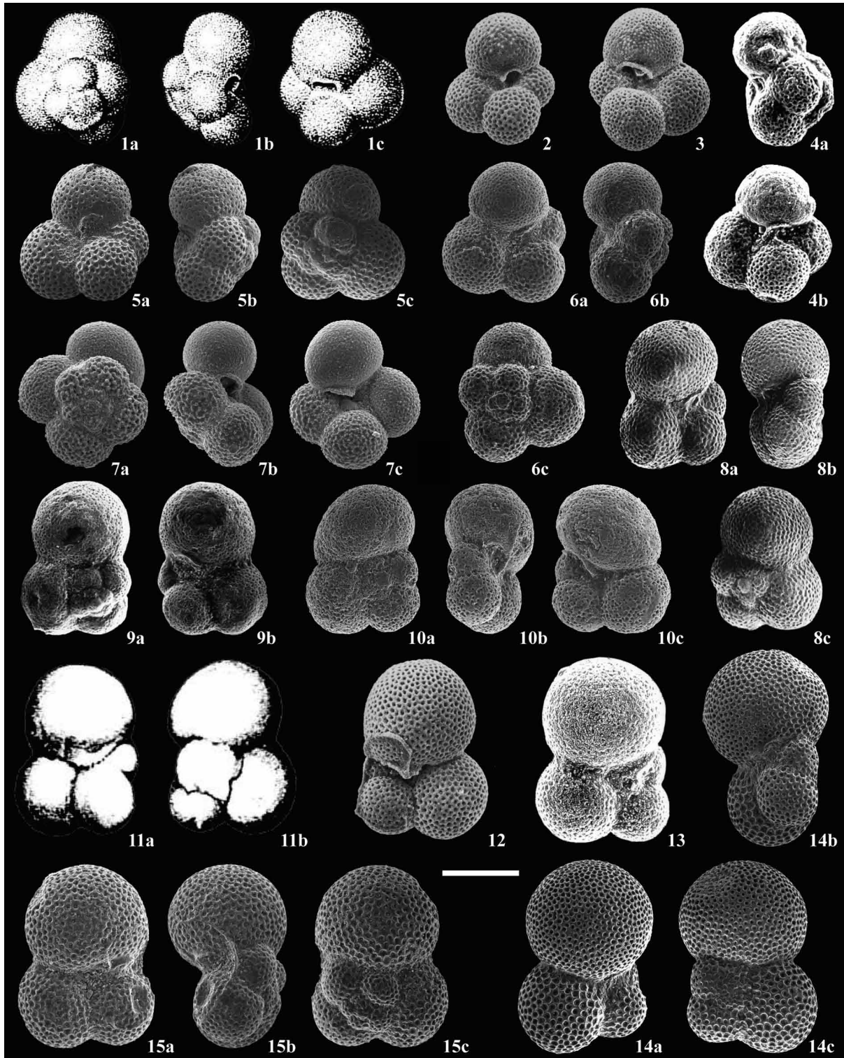
Figure 3. SEM images of Eoglobigerina and Subbotina species (scale bar = 100 \mu m). 1-7. Eoglobigerina cf. trivialis = Eoglobigerina trivialis (Subbotina, 1953), sensu Blow (1979): 1, paratype from the Danian sediments, Kuban River, Northern Caucasus, Russia (from Subbotina, 1953, pl. 4, fig. 6a-c); 2, hypotype from Blow (1979) from the Zone P1, DSDP Leg 6, South Pacific (from Blow, 1979, pl. 73, fig. 3); 3, hypotype from Blow (1979) from Zone P1, DSDP Leg 6, South Pacific (from Blow, 1979, pl. 73, fig. 5); 4, specimen from the S. triloculinoides Subzone, El Kef, Tunisia; 5, specimen from the G. compressa Zone, Caravaca, Spain; 6, specimen from the S. triloculinoides Subzone, Ben Gurion, Israel; 7, specimen from Danian, DSDP Site 305, Shatsky Rise, North Pacific. 8-10. Eoglobigerina microcellulosa (Morozova, 1961): 8, holotype from the lower Danian sediments, Tarkhankhut Peninsula, Crimea, Ukraine (from Olsson et al. , 1999, pl. 9, figs. 13-15); 9, specimen from the G. compressa Zone, Caravaca, Spain; 10, E. microcellulosa , specimen from the E. simplicissima Subzone, El Kef, Tunisia. 11-15. Subbotina triloculinoides (Plummer, 1927): 11, holotype from the Danian sediments, Station 23, continues
