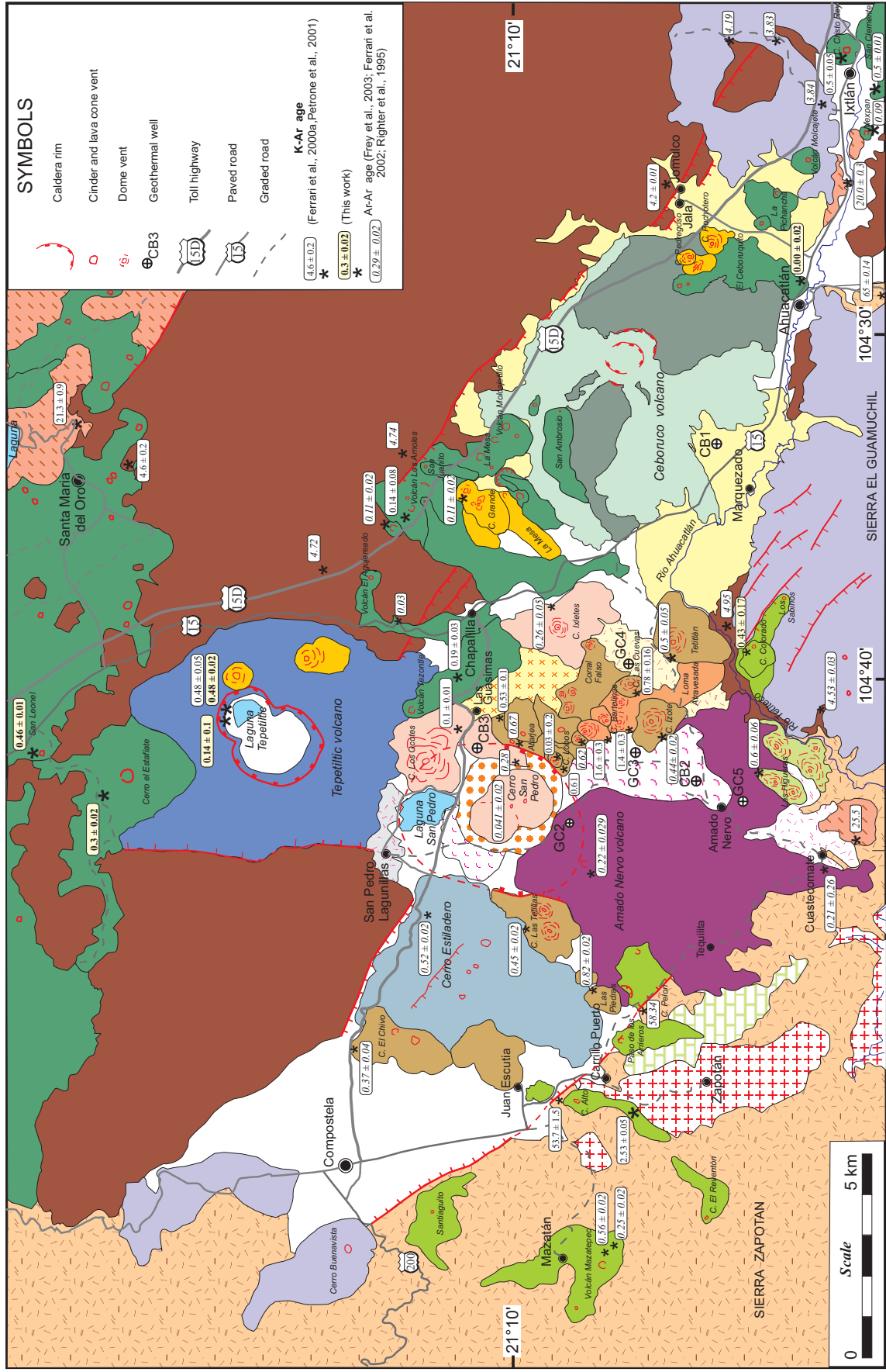
Figure 6. Geologic map of the San Pedro - Ceboruco area.
