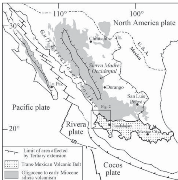
Figure 1. Geodynamic map of Mexico showing Tertiary extension and volcanism north of the Trans-Mexican Volcanic Belt and the present configuration of plates. The area of Figure 2 is boxed. Tertiary extension according to Ferrari et al. (2002).
